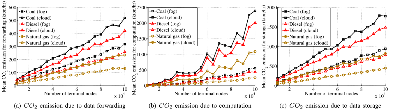
Fig. 7. Analysis of \text{CO}_2 emission for non-renewable energy sources.
